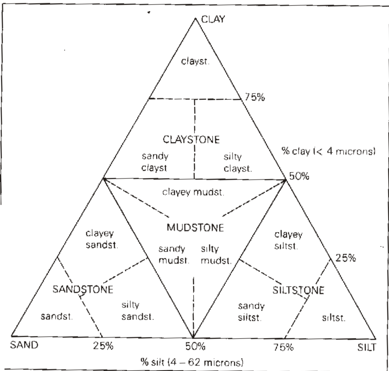
Fig. 3.2 Scheme for describing sedimentary rocks of sand-silt-clay grain sizes (after M. D. Picard).
