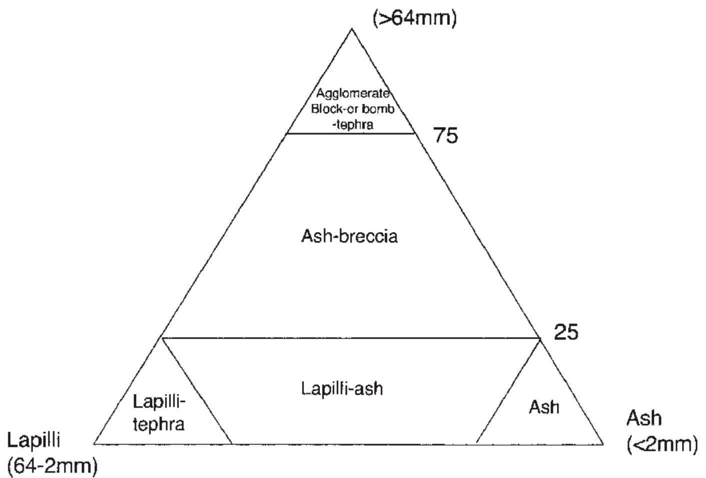
Classification of tephra
