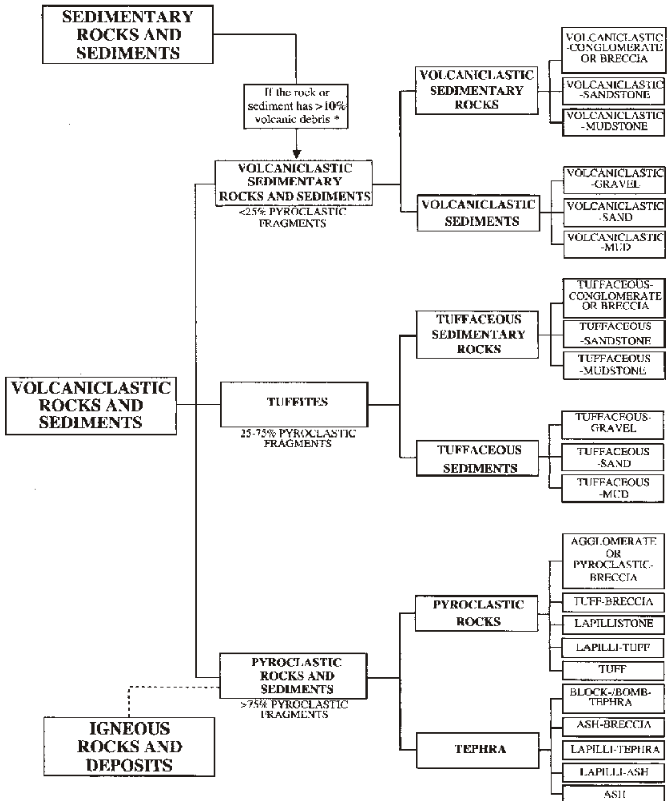
FIGURE 4. HIERARCHICAL CLASSIFICATION OF VOLCANICLASTIC ROCKS AND SEDIMENTS
