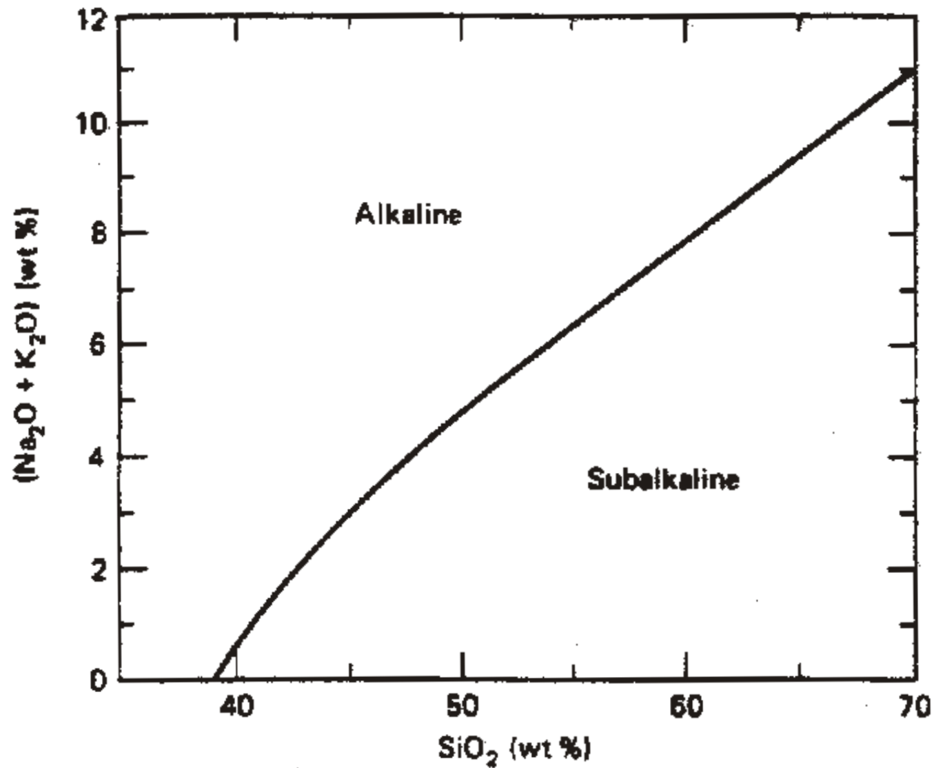
FIGURE 6-6 Alkalis-silica plot with line separating fields of alkaline and subalkaline rocks. [After Irvine and Baragar (1971).]
