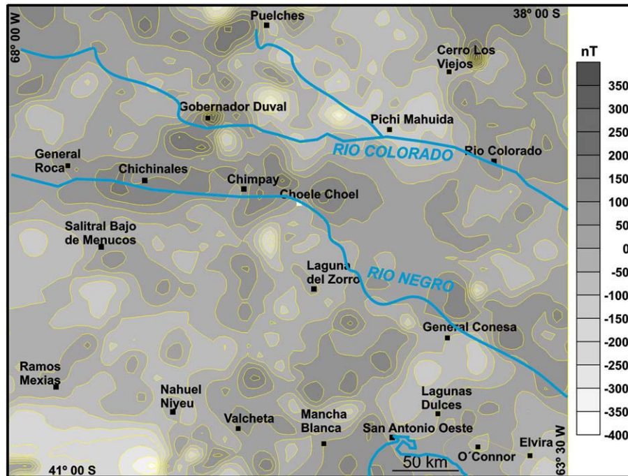
Fig. 9. Map showing distribution of the magnetic anomalies. No obvious correlation with Bouguer anomalies was observed. Most anomalies are discontinuous and segmented.
