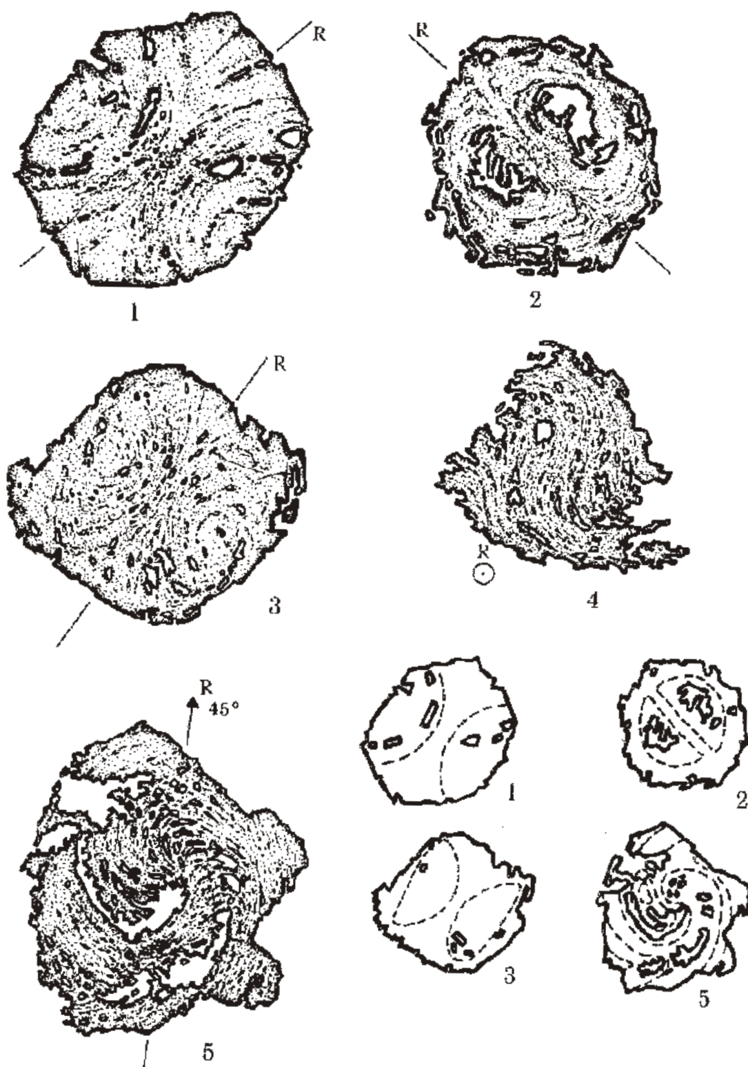
Fig. 5.16. Various facies of helicitic inclusions in synkinematic garnets: (1) pc inclusions; (2) op inclusions; (3) pu inclusions; (4) and (5) spiral inclusions (R = rotation axis, \phi \approx 0.5 cm).
