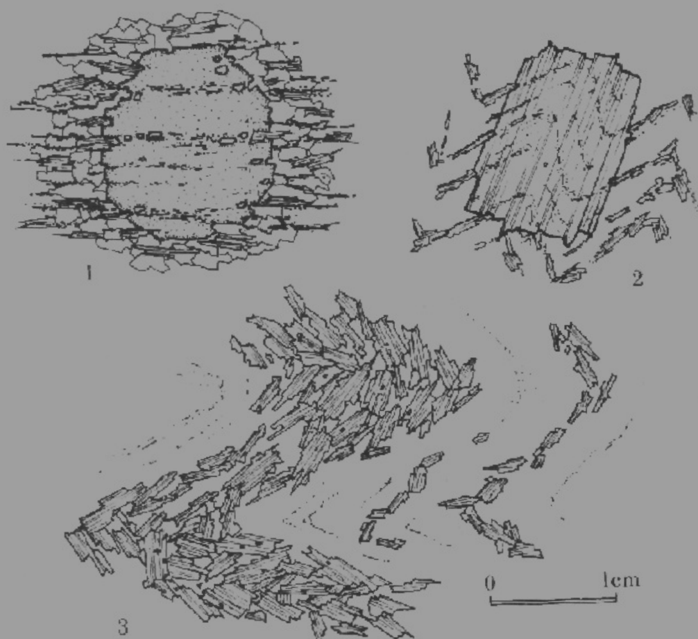
Fig. 5.12. Various habits of postkinematic minerals: (1) ' static ' blast on a flow schistosity S_n (or S_{n+1} ); (2) ' static ' blast on a strain-slip cleavage (at least 2 tectonic 'phases' before the mineral growth); (3) ' polygonal arch ' with phyllosilicates mimetic of a microfold anterior to their own static (re)crystallization).
