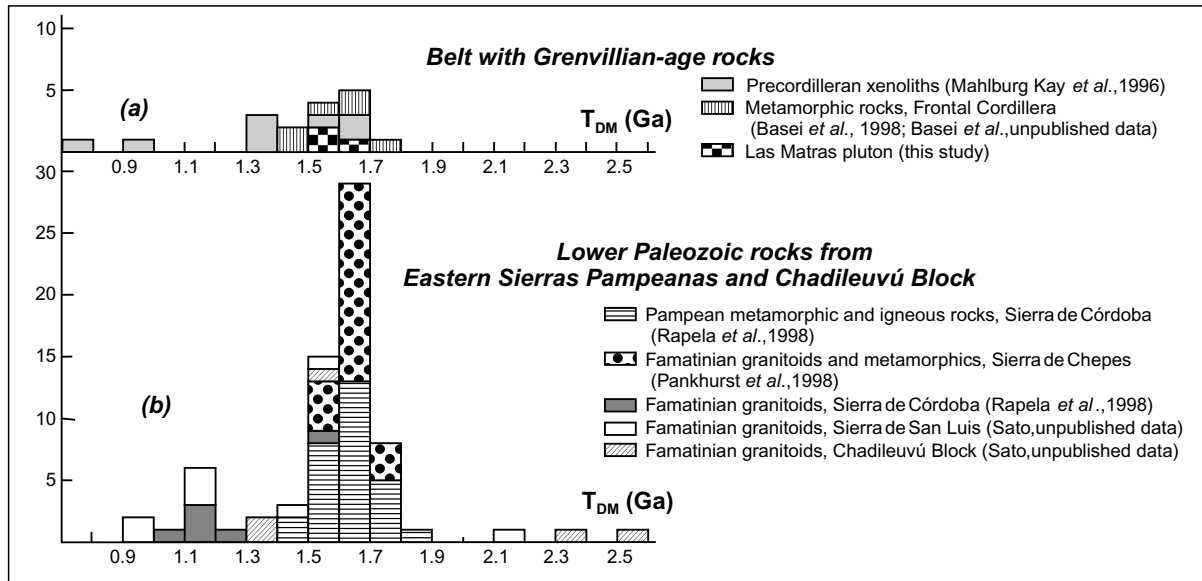
Fig. 11. T_{DM} model age histograms for: (a) the Grenvillian-age basement rocks (17 samples); and (b) the Early Paleozoic basement rocks from the Eastern Sierras Pampeanas and the Chadileuvú Block (70 samples). Although the orogenic cycles involved in these two parallel belts are different, the compiled T_{DM} data do not suggest, up to now, a clear separation of the lower crustal compositions of both belts. Only some few Paleoproterozoic data are remarkable in the Eastern Sierras Pampeanas and the Chadileuvú Block, which are not seen in the Grenvillian-age rocks.
